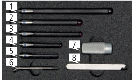
Styli Kit 1 VAST XXT, for small workpieces 형식 : 626103-9021-000*
