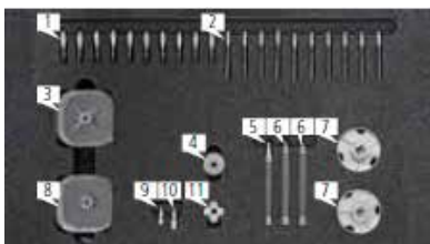
Star stylus kit XXT TL3 gear measurement 형식 : 626103-9034-000
