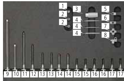
VAST XXT styli kit 5, large 형식 : 626103-9025-000
